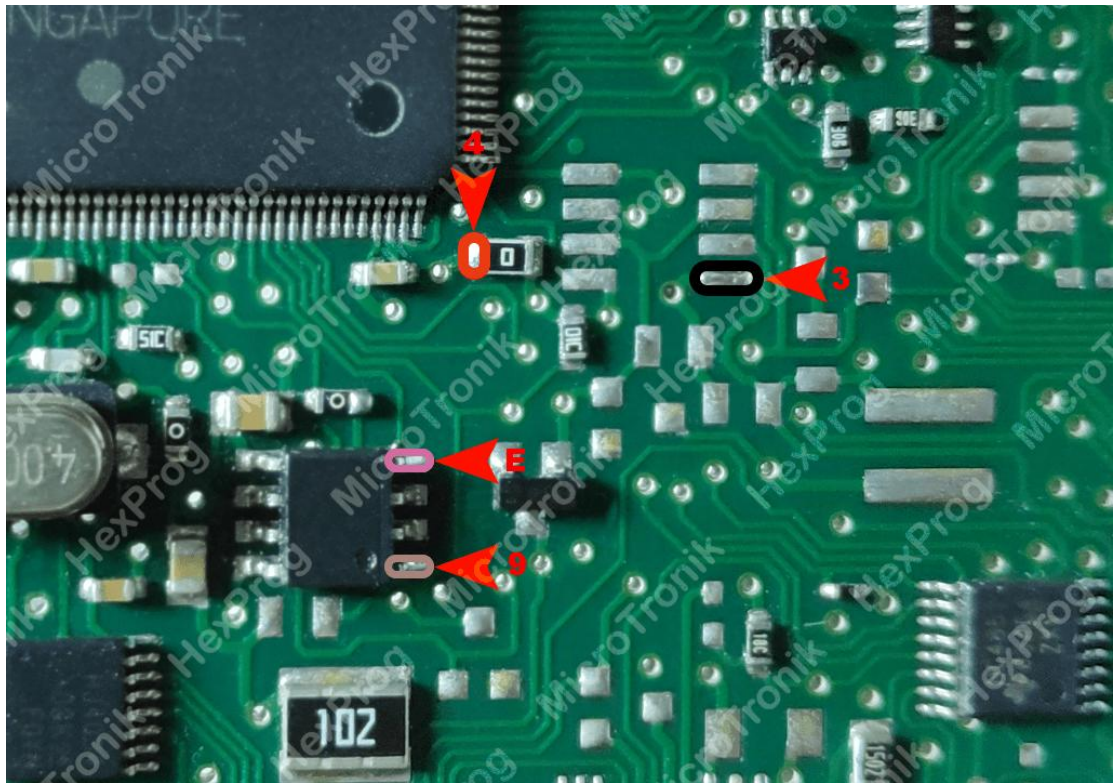
Audi BCM2 Front Wiring
